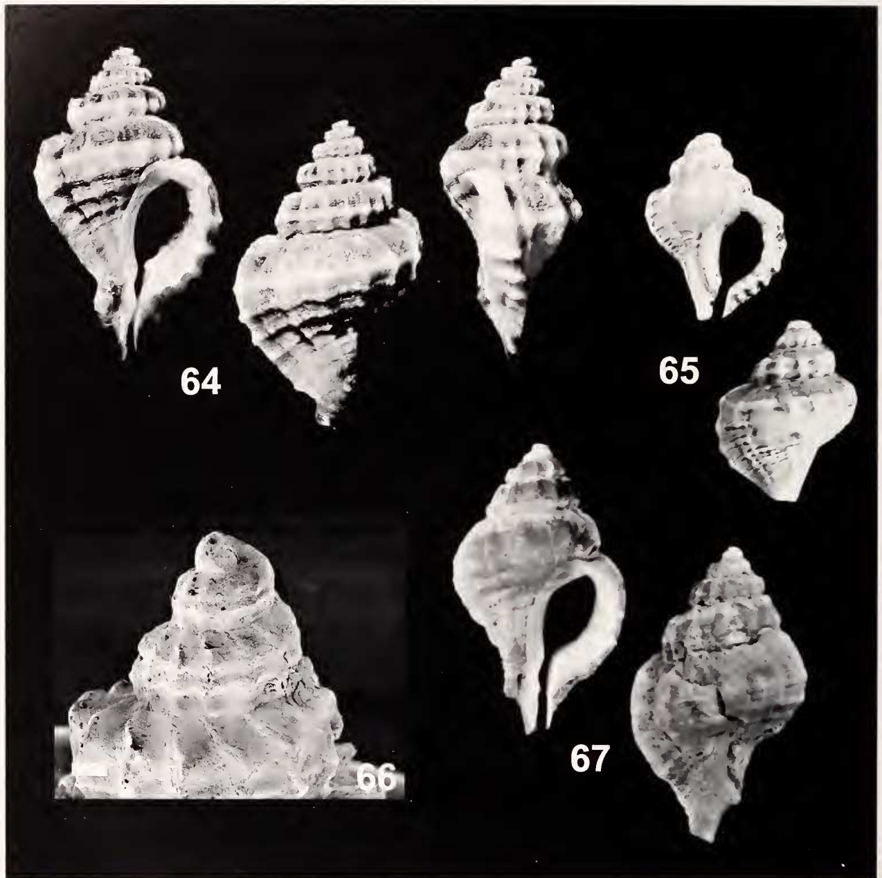
Figures 64–67. Eupleura plicata (Reeve, 1844). Figure 64. UMCZ 1.100.275, J. Saul Collection (Holotype); locality: unknown (fide Reeve, 1844a); height 34.2 mm, diameter 20.0 mm. Figure 65. USNM 162559 (Holotype of Eupleura muriciformis var. curta Arnold, 1903); locality: San Pedro, California; Pleistocene, Upper San Pedro Series; height 15.0 mm, diameter 10.0 mm. Figure 66. ANSP 115981; locality: Archipelago de las Perlas, Panama; scanning electron micrograph of the early teleoconch whorls (scale bar = 200 \mu m). Figure 67. UF 267562; locality: Archipelago de las Perlas, Panama; height 35.5 mm, diameter 21.0 mm.
